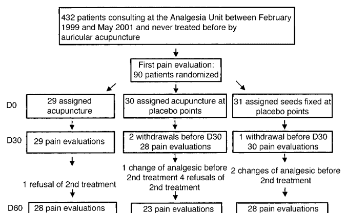
Fig 2. Trial profile.
